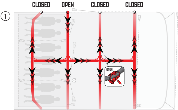
SINGLE POINT INFLATION: OPERATE SELECTED VALVE AND KEEP ALL CONNECTING TUBES OPEN
