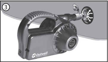
When fully inflated seal valve by pushing in the pump nozzle. This will seal the internal stopper and keep air from escaping while closing cap.
